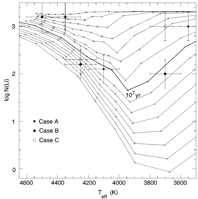
FIG. 4.—Evolution of the surface Li abundance as a function of T_{\text{eff}} . Isochrones are equally spaced in time by 1 Myr, starting with 3 Myr at the top to 17 Myr at the bottom. The heavy line corresponds to 10 Myr. Uncertainties are approximately 0.3 dex in the Li abundance and 100 K in T_{\text{eff}} . The squares correspond to case A, the solid circles to case B, and the open circles to case C.
